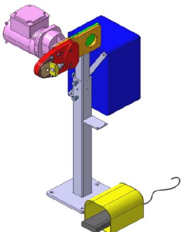
set-up variant V1 (F-3500.037.001)
